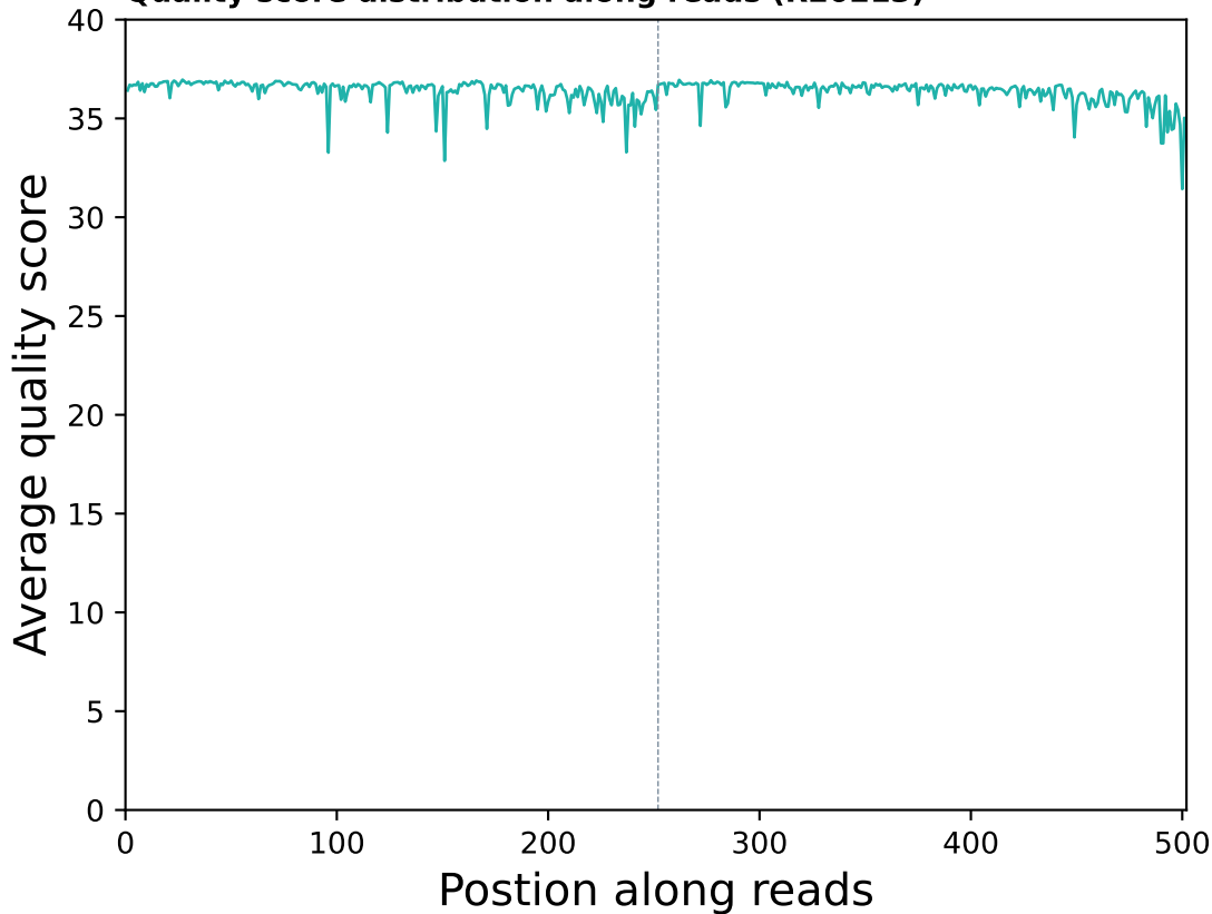
Quality score distribution along reads (R20213)
